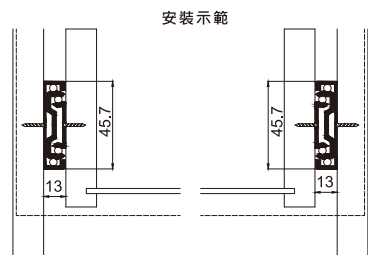
安裝寬度 13mm, 誤差調節+0.2mm Width 13mm Error Adjustable Flat Screw+0.2mm
