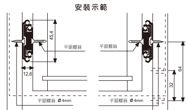
安裝寬度 12.6 mm, 誤差調節+0.2mm Width 12.6 mm Error Adjustable Flat Screw+0.2mm
