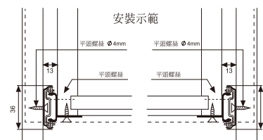
安裝寬度13mm，誤差調節+0.2mm Width 13mm Error Adjustable Flat Screw+0.2mm
